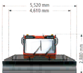
PistenBully 600 Polar
